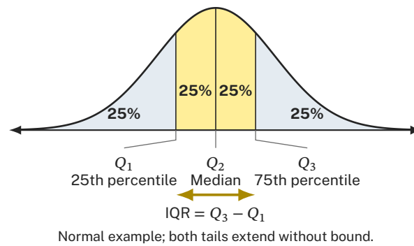
Figure 7. Quartiles and the interquartile range on a normal curve
